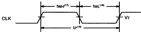
Clock Width/Period
