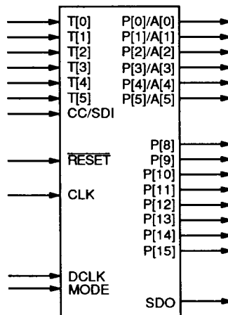
SSR® Diagnostics Configuration
