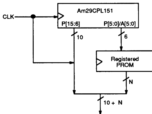
Figure 2. Controlling External PROM
