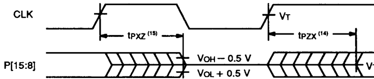
CLK to Output Disable/Enable
