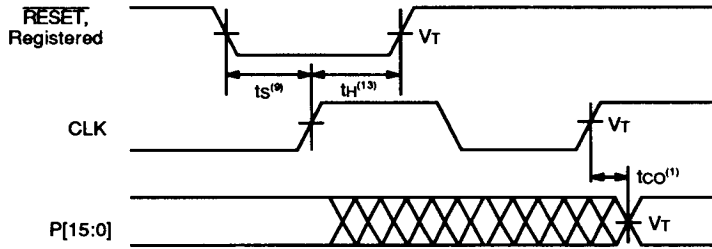
Registered RESET
