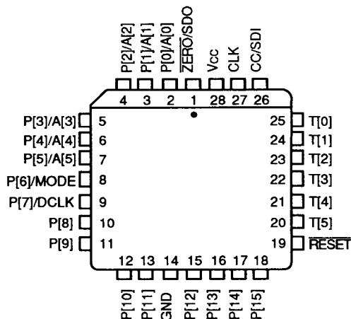
PLCC/LCC
