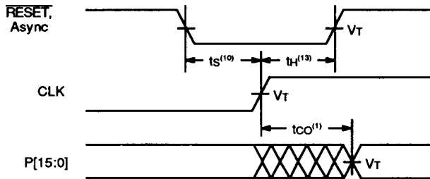
Asynchronous RESET
